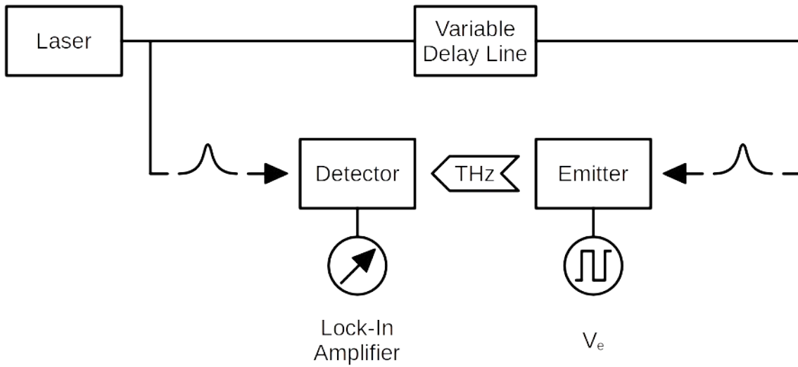
Figure 1: Setup for THz measurements
